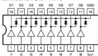
PIN CONNECTION (TOP VIEW)
