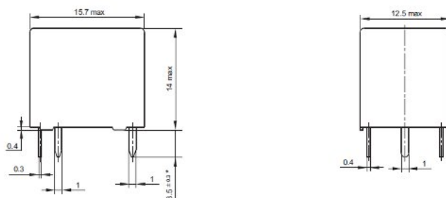
Outline Dimensions(1 Form A / 1 Form C)
