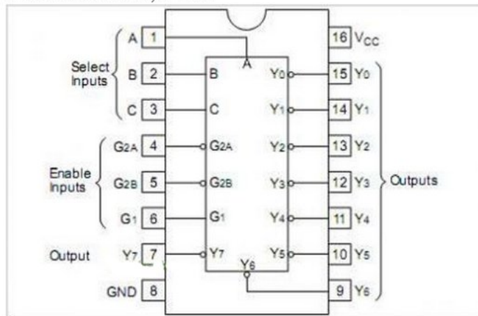
HD74HC138 Pinout, Pinouts
